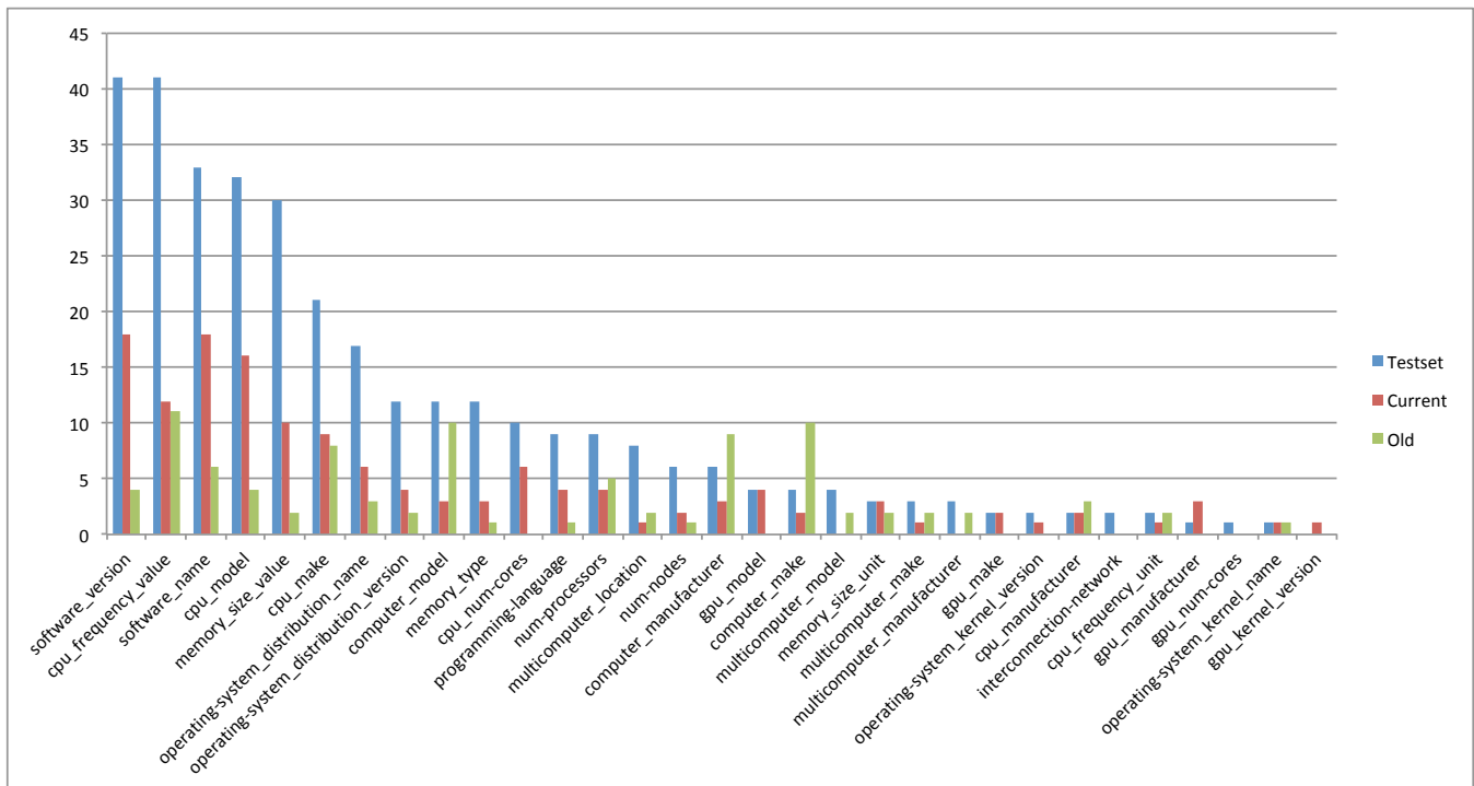
Figure 2: The number of distinct values for each tag in the test set and the current and old training sets.
