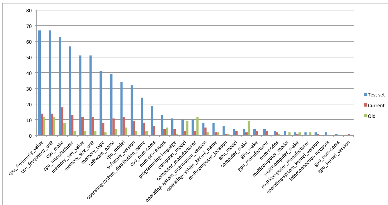
Figure 3: The number of occurrences of each tag in the test set and the current and old training sets.
