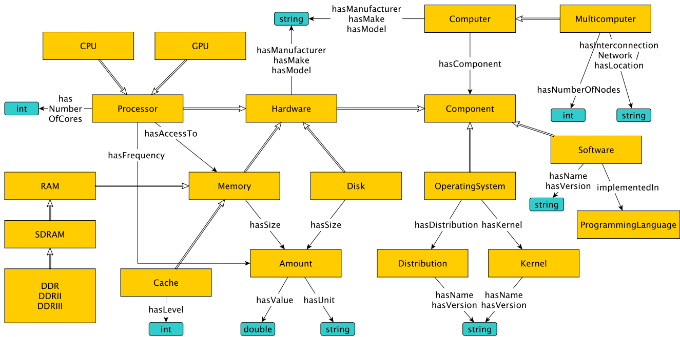
Figure 1: The Computational Environment ODP
